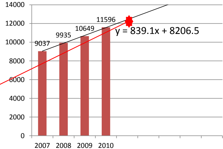
Linear Model prediction
