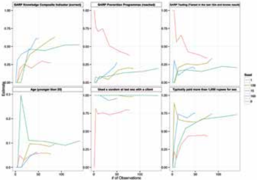
Figure 11: Bottleneck plots, FSW Kandy
