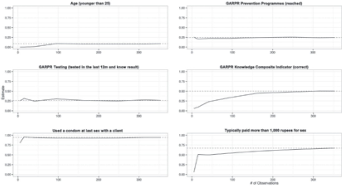
Figure 10: Convergence on key indicators, FSW Kandy
