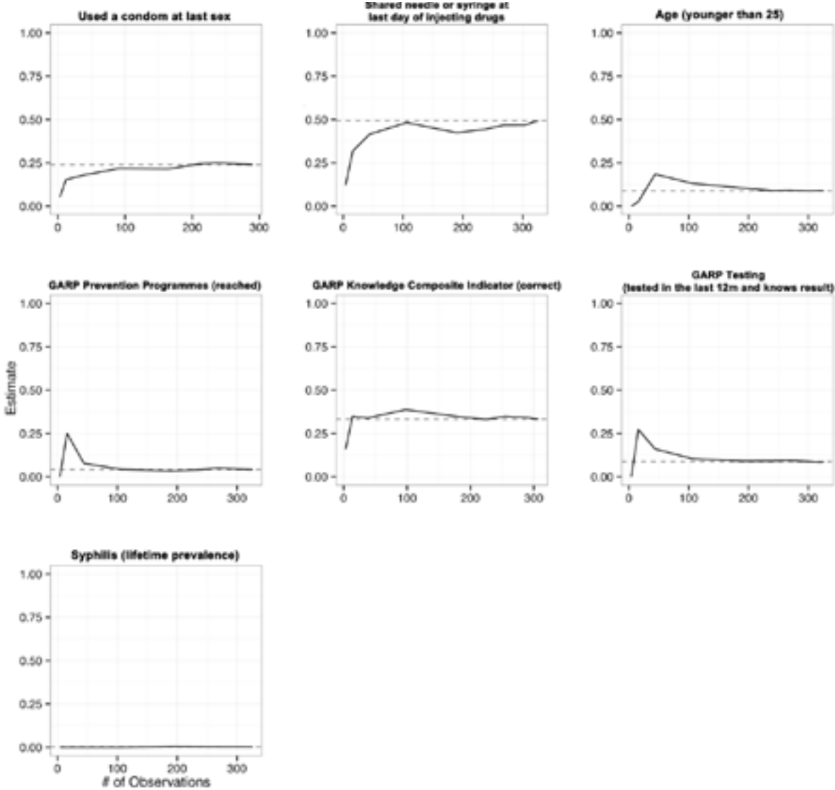
Figure 23: Convergence on key indicators, PWID Colombo
