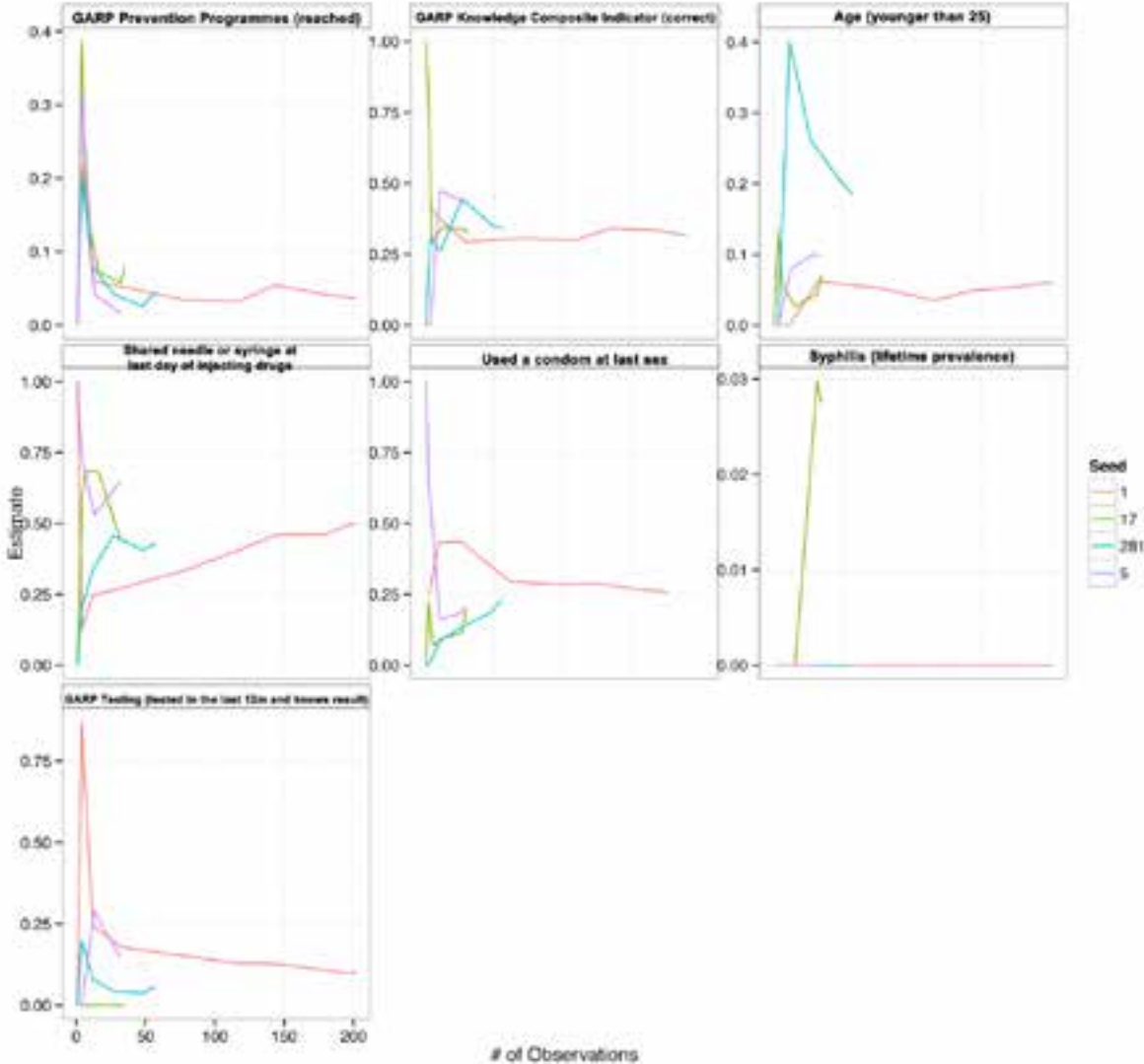
Figure 24: Bottleneck Plots, PWID Colombo
