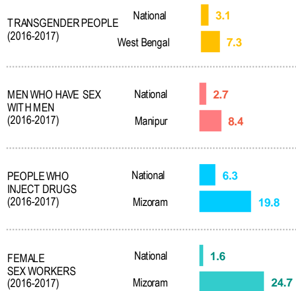
Source: Serological surveys and Global AIDS Monitoring 2018
